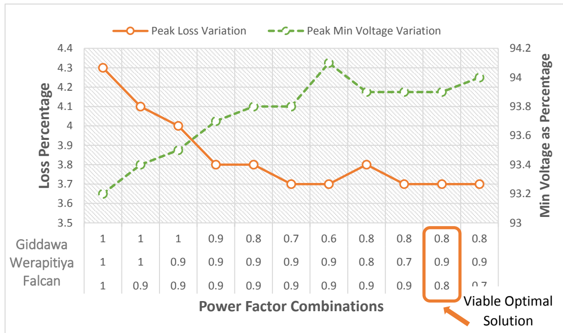
Figure 3.5: Loss and Minimum Voltage Variation along Feeder at Peak
