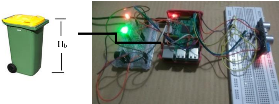
Fig. 5. IOT Module Integrated to the Smart Waste Bin
