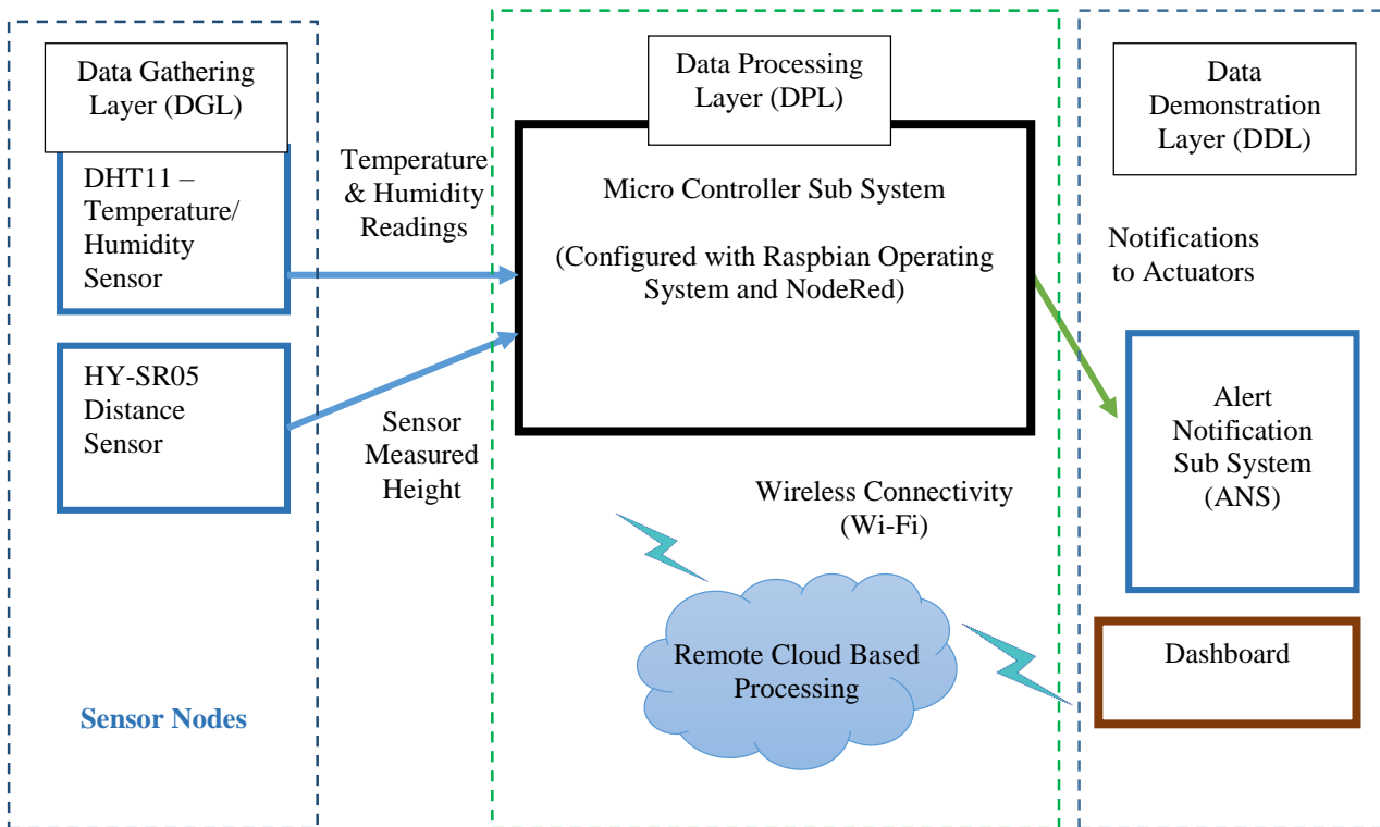
Fig. 1 System Overview of IOT based Smart Waste Bin Model
