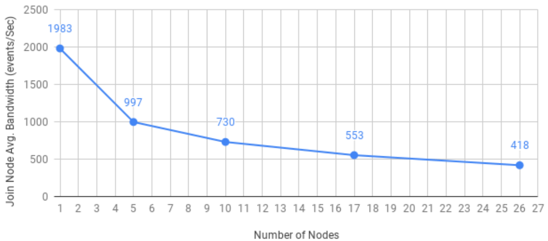
Fig. 5.17: Average join node bandwidth while holding the largest possible length window.
