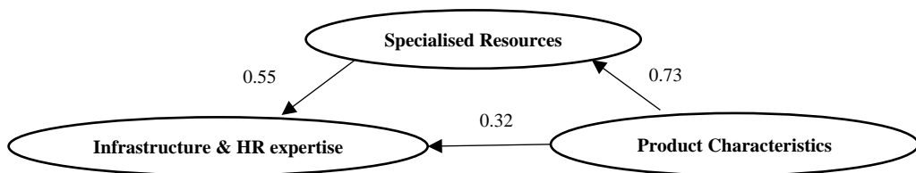
Figure 2: Output from the Accepted model of SEM
