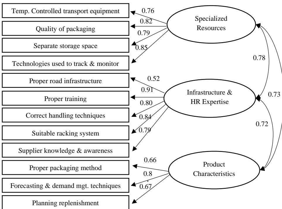
Figure 1: Output from the accepted model of CFA
