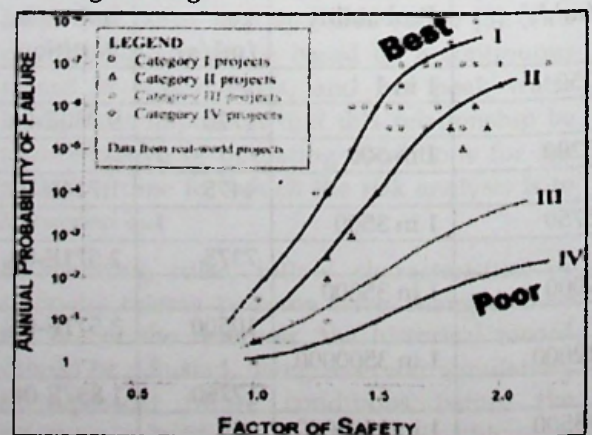
Figure 2: Factor of safety versus annual probability of failure [6]
